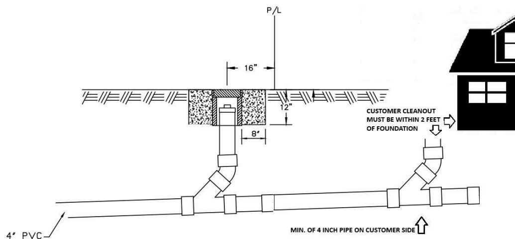
CLEAN-OUT DETAIL
